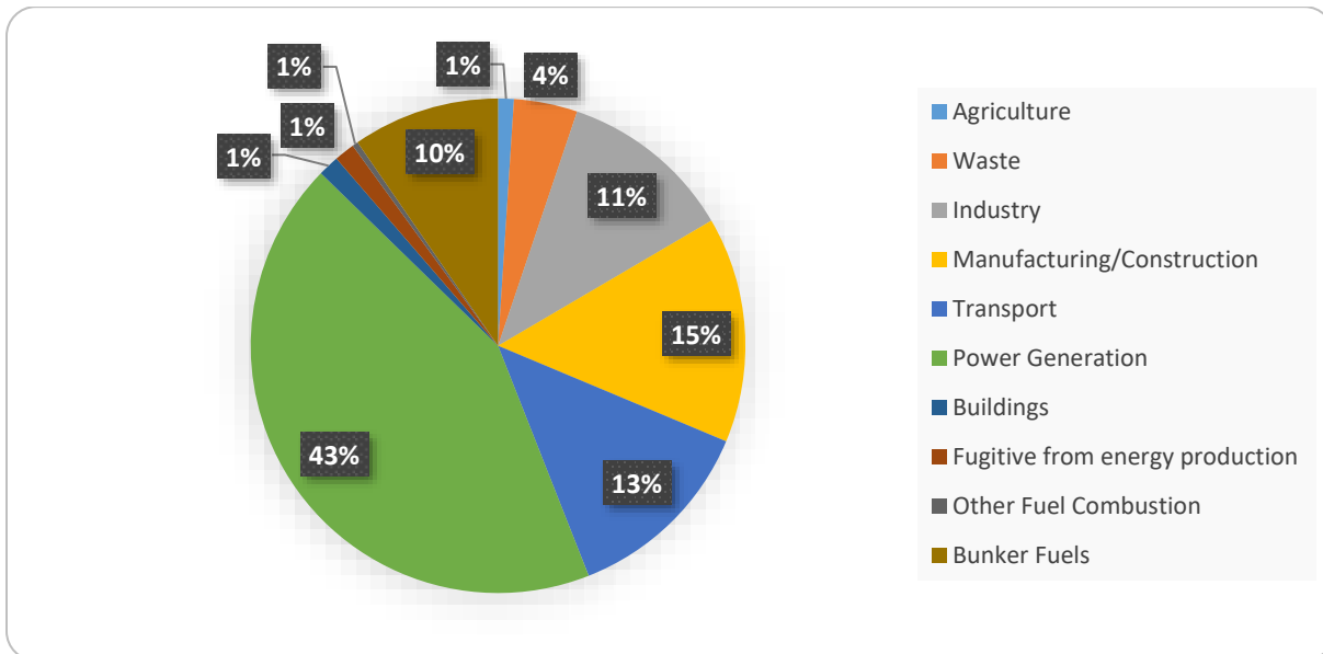
Chart 3 GHG (MtCO 2 e) Emissions by Sector (2020) *
