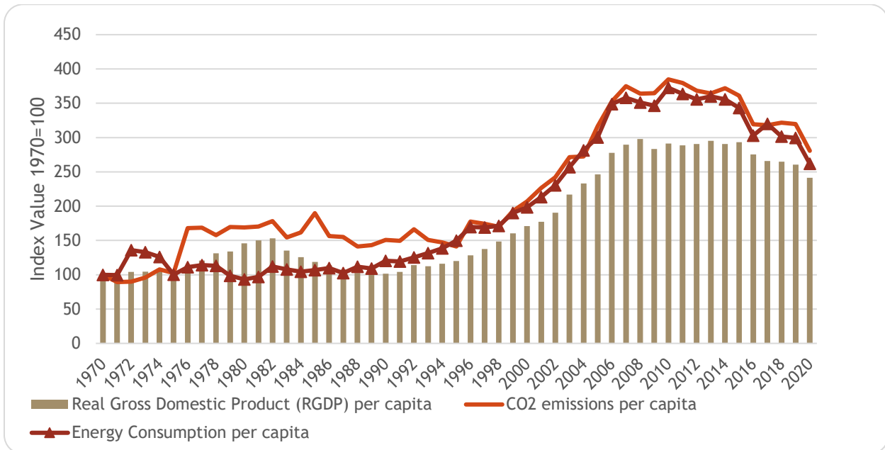
Chart 2 Annual Carbon Dioxide (CO 2 ) Emissions, GDP and Energy Consumption
